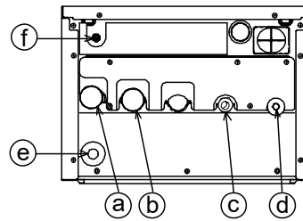
Pipe Position Diagram
